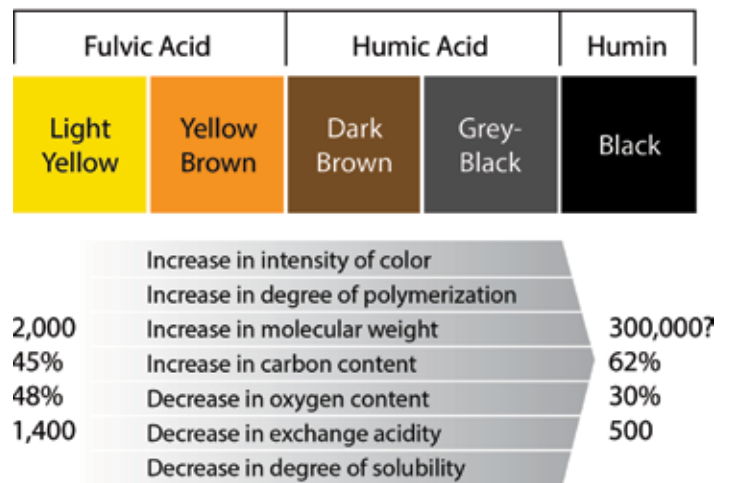
Figure 1. Chemical Properties of Humic Substances 4
