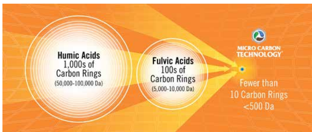
Figure 2. Molecular Size Comparison of Humic Acids, Fulvic Acids, and Micro Carbon Technology®
